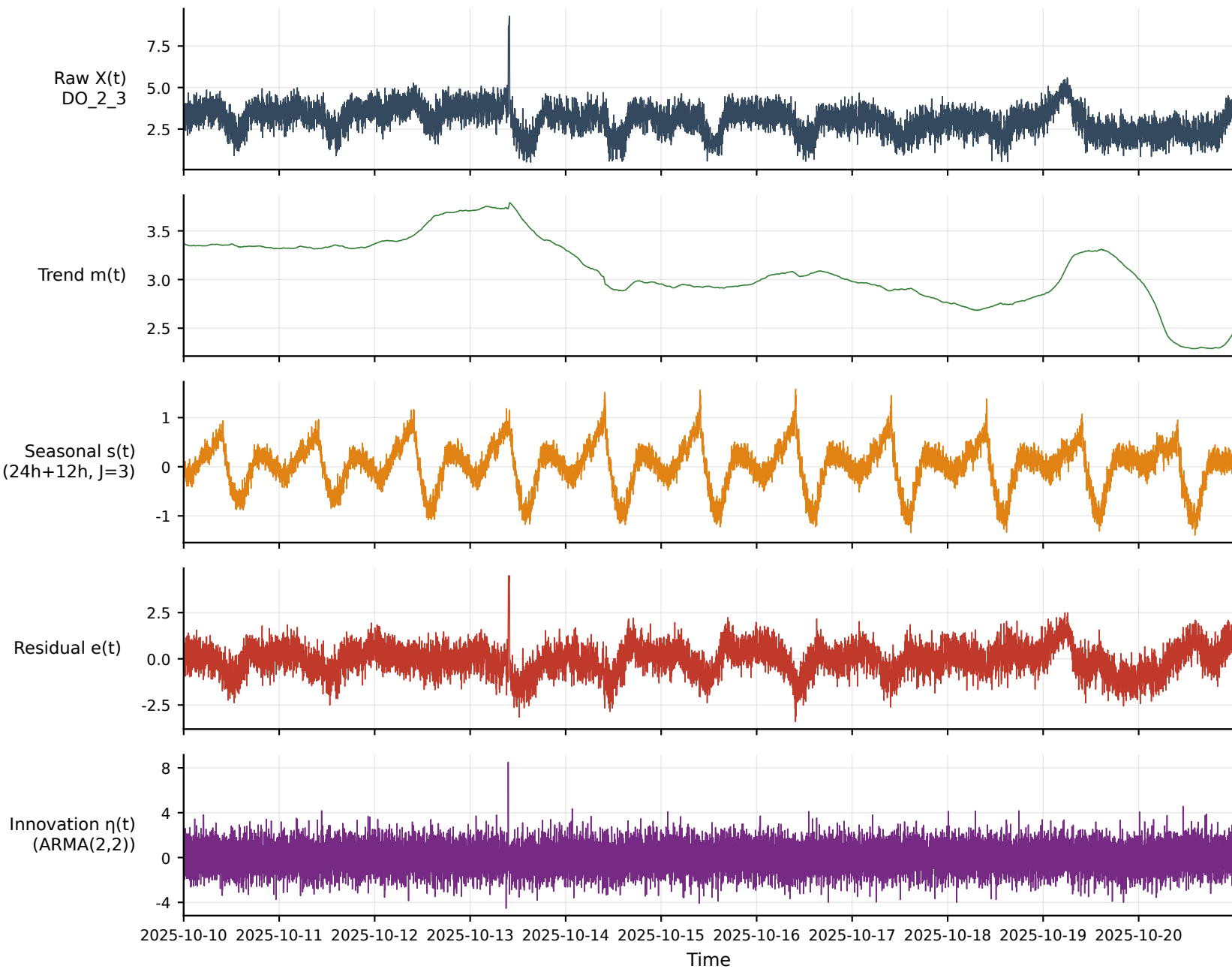
Multi-scale decomposition — DO_2_3 (aerobic, min) [2025-10-10~2025-10-20]
